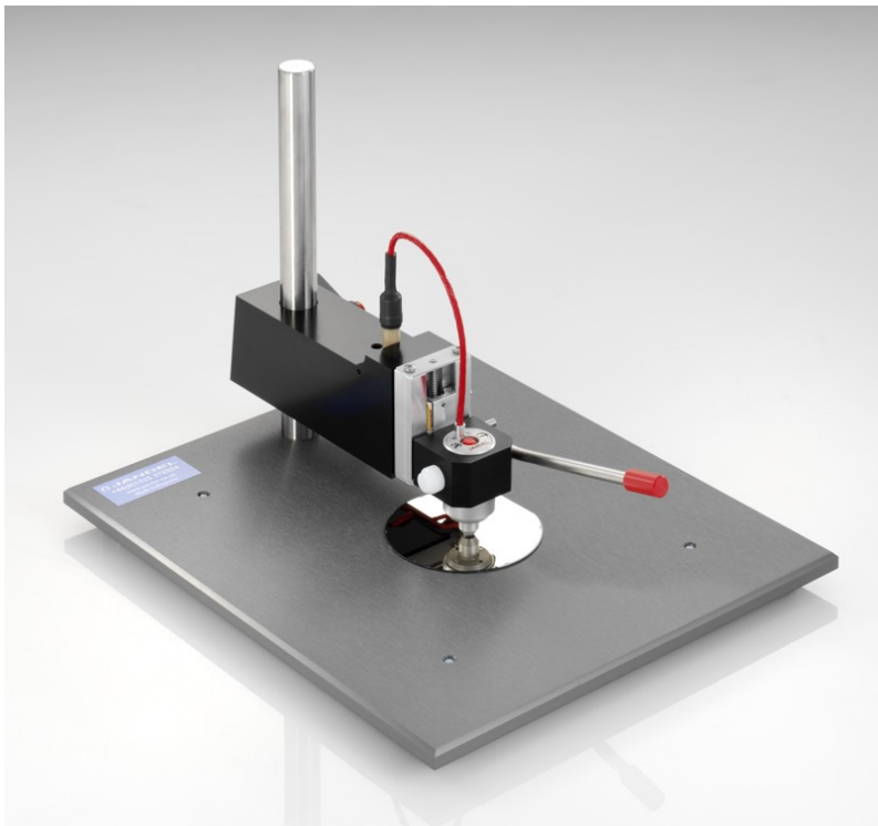
X-Y stage removed, probing 3" wafer
